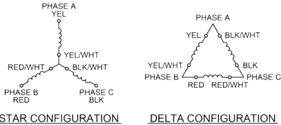
STAR CONFIGURATION
